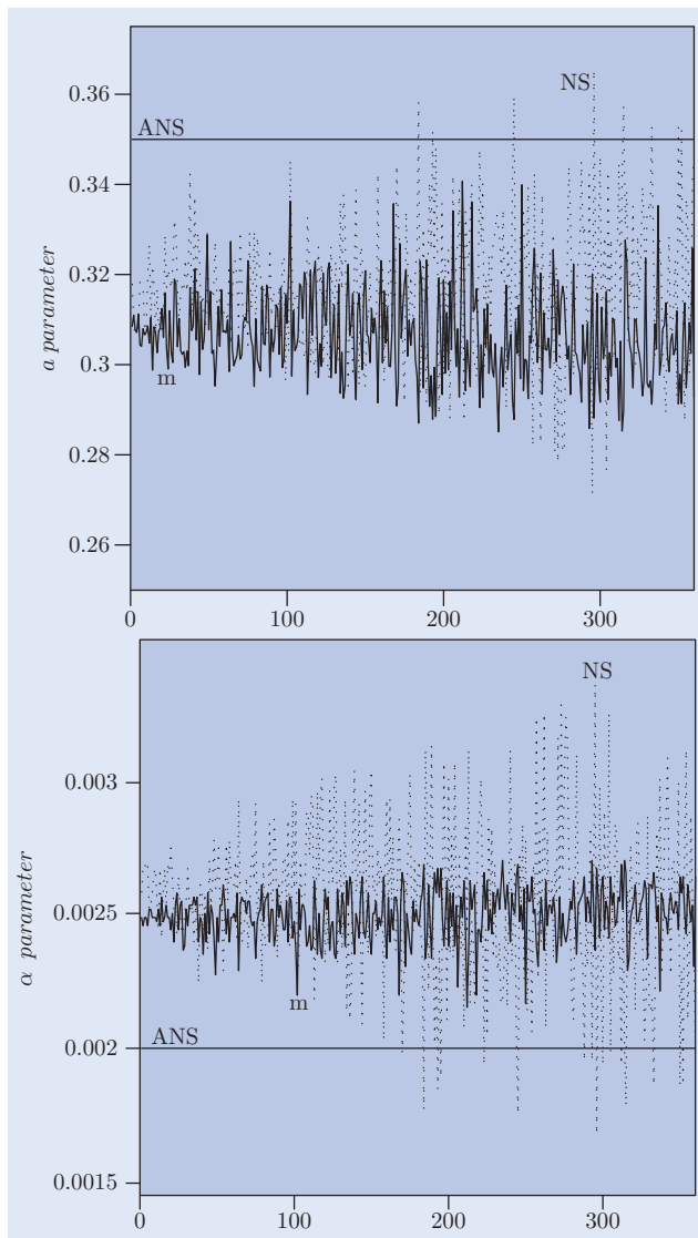
Figure 3. Daily estimates of parameters a and \alpha for data simulated from the model with \alpha=0.002 and a=0.35 and starting forward curve r_0(x)=r_{\text{ANS}}^*(x) . The straight line corresponds to daily calibration results for the ANS family, the irregular line for the MC family and the dashed line for the NS family.
