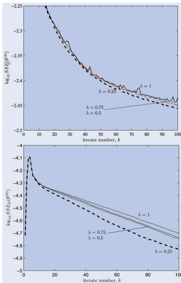
Figure 2. Convergence properties for the joint calibration algorithm for the MC family. SSE_C and SSE_D contributions to the total loss function. We present the mean of the path iterates generated by 1000 uniformly distributed choices of the initial seed, \theta^{(0)} .
