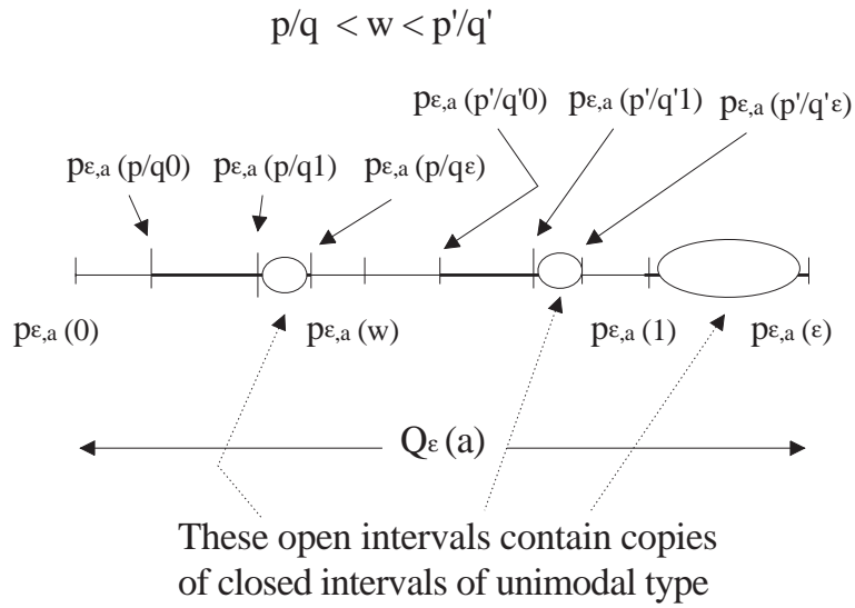
Fig. 2. The description of the closed interval Q_\epsilon(a) using the map p_{\epsilon,a} . Note that the gaps also contain the sequences with unbounded symbols.
